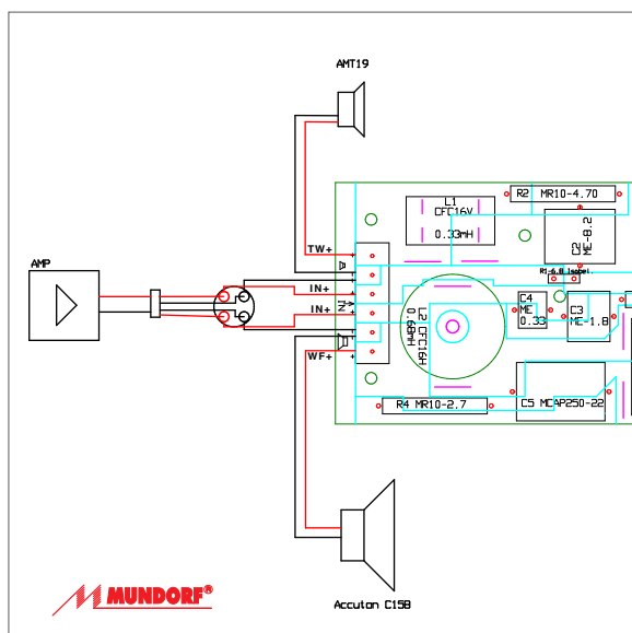
Bi-Wiring/-Amping • MA30 Kit X-Over-Layout
