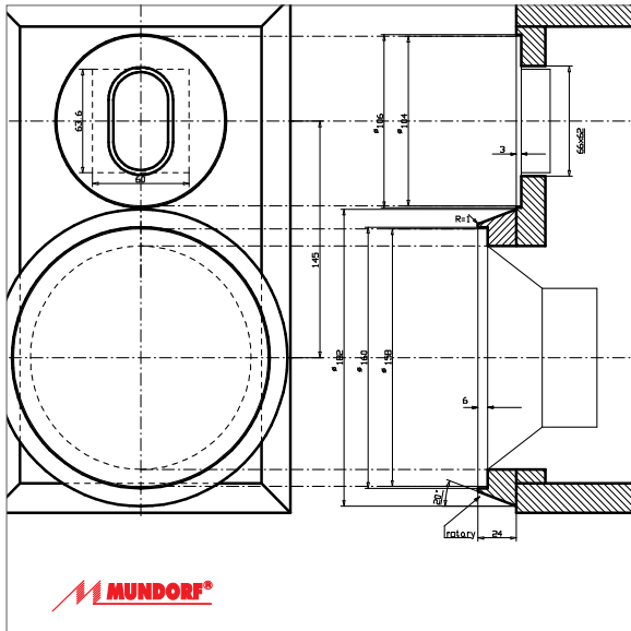
Extended Baffle • Cabinet Drawing Available
