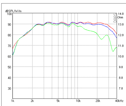
SPL Horizontally 0° - 15° - 30°
